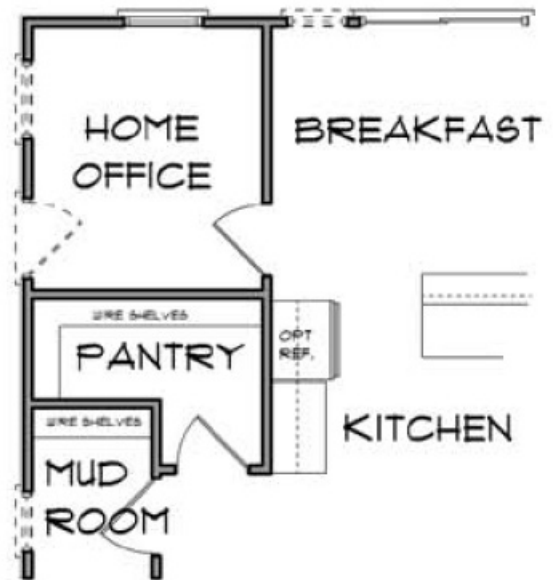
OPTIONAL HOME OFFICE EXTENSION
